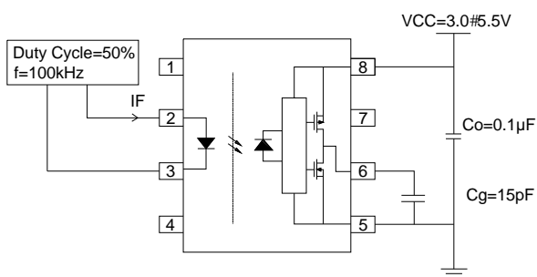
Fig.9: Test Circuits for TPHL, TPLH, tr, tf
