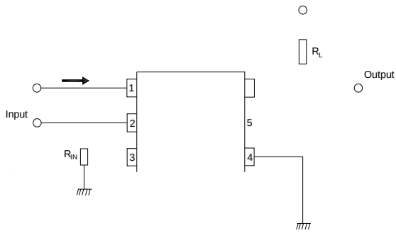
Test Circuits of Turn On Time
